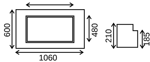
9816 Louvre Aircon holder
