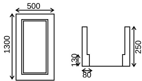
9758 Louvre vent 1300x500
