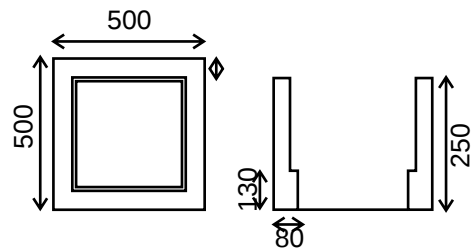
9759 Louvre vent 500x500
