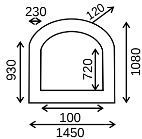
9760 JIC vent large
