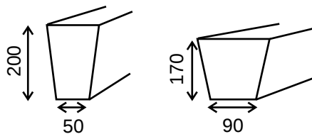
9141 Lintol 50 x 200 x 500mm 9166 Lintol 90 x 170 x 2400mm
